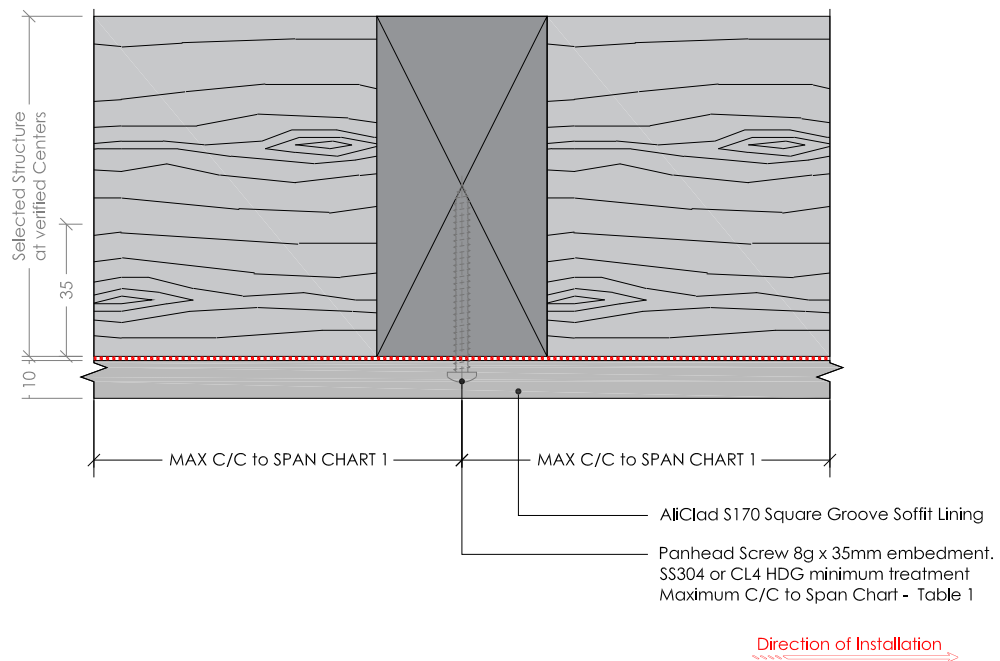
2 Intermediate Board Fixings Parallel Section 1:2 @ A4
