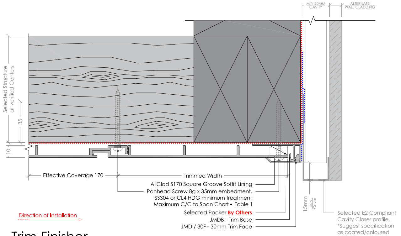
1 Trim Finisher Perpendicular Section 1:2 @ A4
