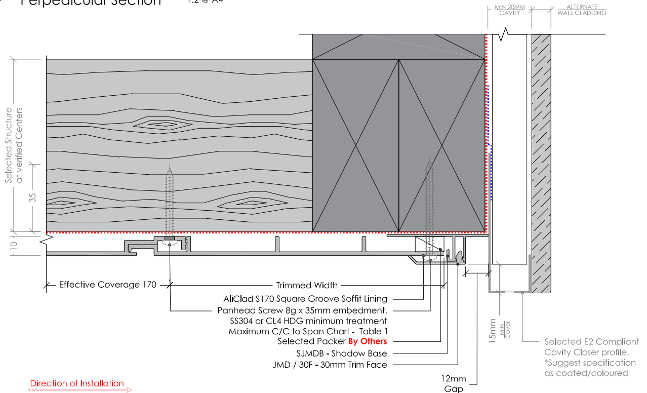
2 Shadow Finisher Perpendicular Section 1:2 @ A4
