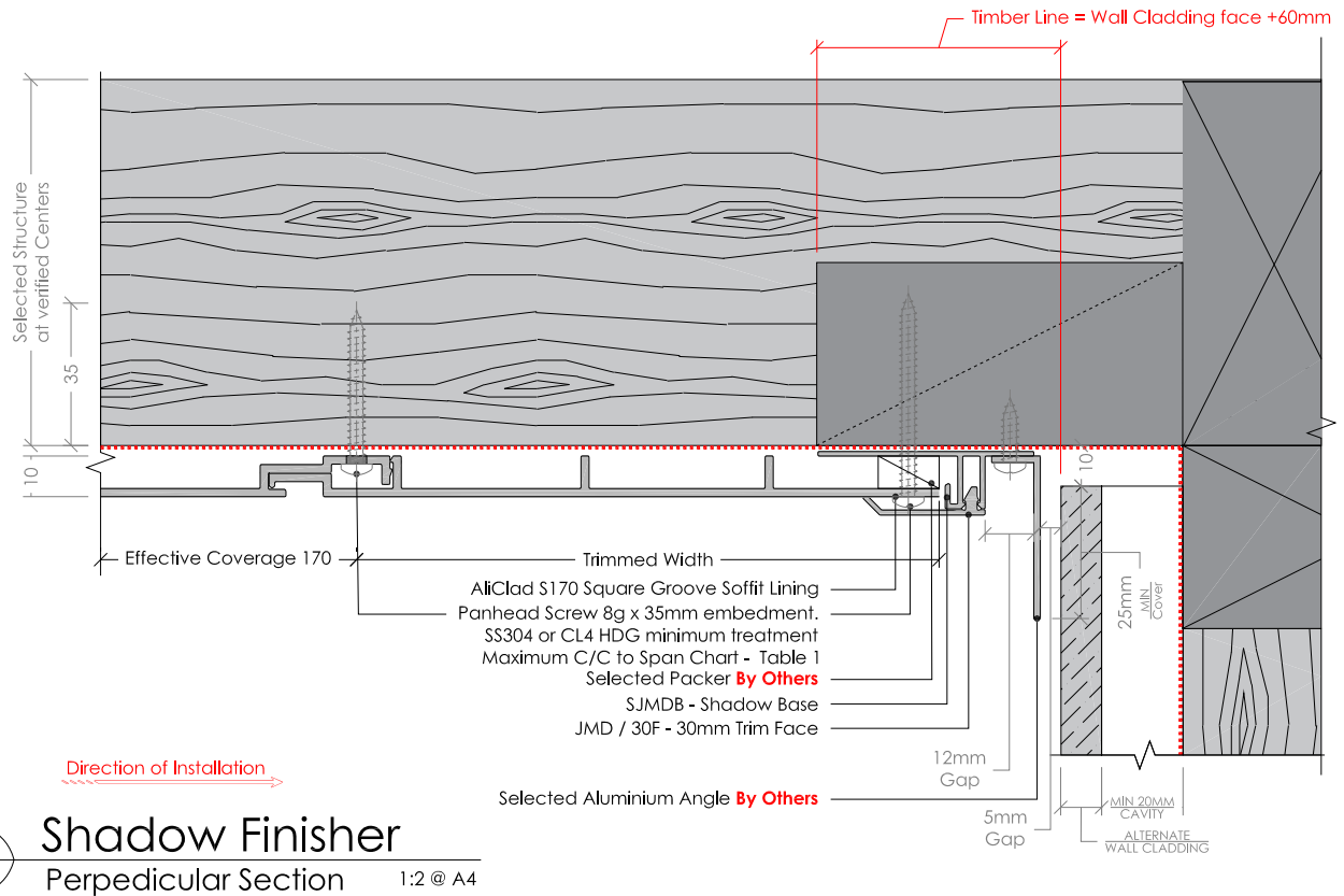
1 Trim Finisher Perpendicular Section 1:2 @ A4
