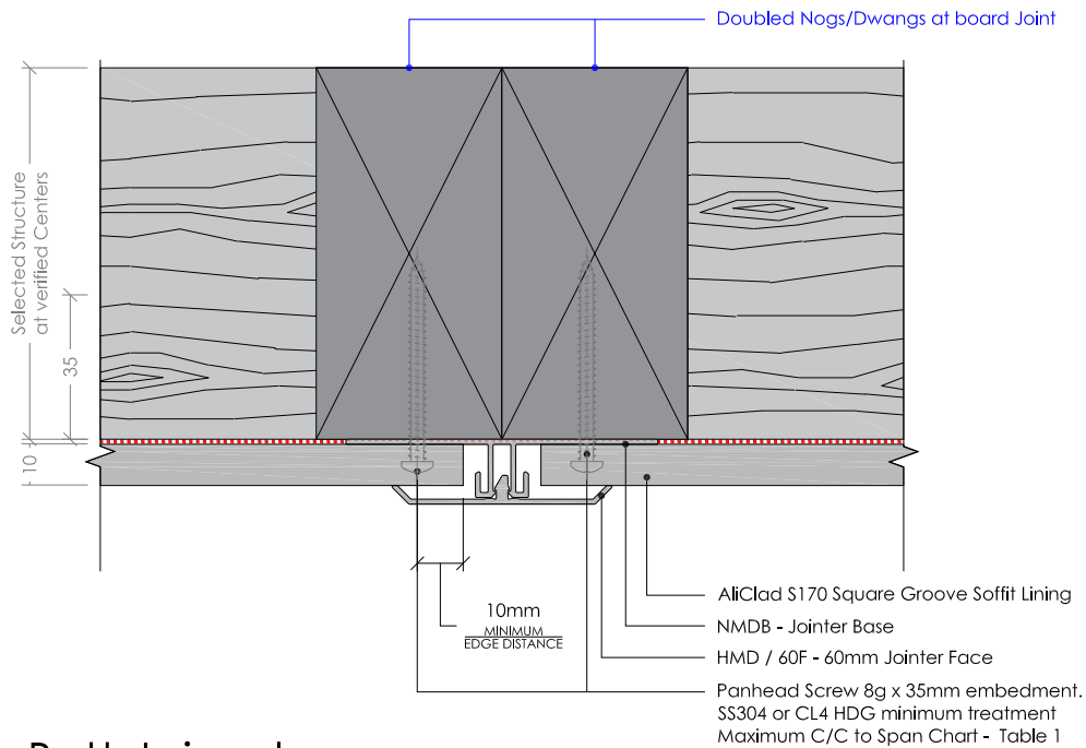
Butt Joined Parallel Section
