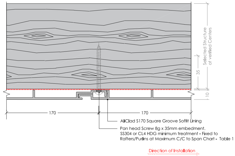
1 Typical Board Connection Perpendicular Section 1:2 @ A4
